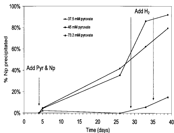
Figure 2. Fate of Np in the growth experiments in which 20 mM sulfate was present. Np precipitation was inhibited by the highest total pyruvate addition. The addition of hydrogen appeared to stimulate Np precipitation.
