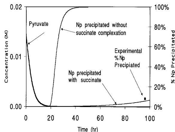
Figure 8. Model-calculated Np(IV) precipitation with and without Np(IV) complexation by succinate. Slow degradation of the intermediate could account for the delayed Np precipitation observed when pyruvate was added as a supplemental electron donor.
