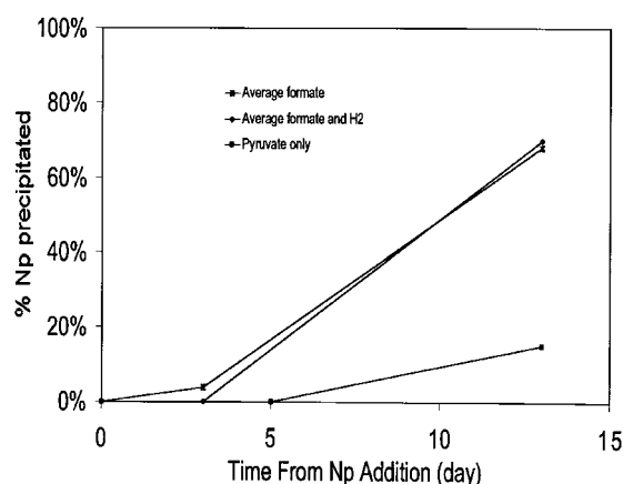
Figure 4. Comparison of Np precipitation by cultures grown on pyruvate and then supplemented with formate, formate + H 2 , or pyruvate alone at time = 0. Np(V) also was added at time = 0. Formate appeared to show the same stimulatory role toward Np precipitation.
