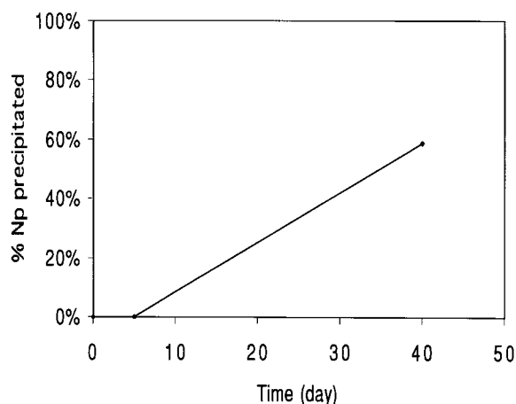
Figure 1. Loss of Np from solution in an anaerobic consortium growing on 10 mM pyruvate in the absence of sulfate. The Np was added after 1 day of growth. An additional 11 mM of pyruvate was added after 13 days. The line is used only to help visualize the results and does not imply a linear trend between 5 and 40 days.
