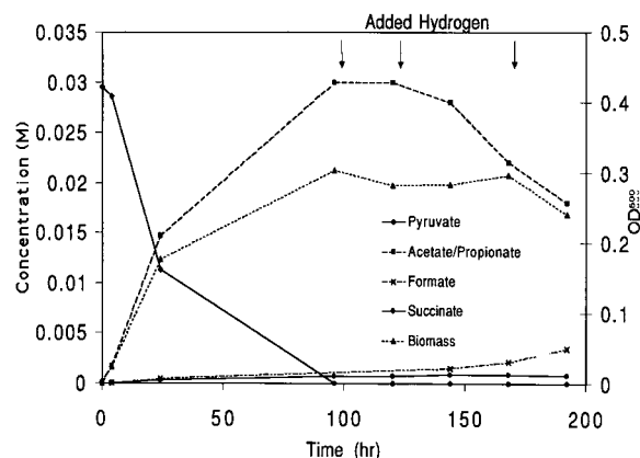
Figure 5. Concentration of major metabolites and intermediates during pyruvate degradation by the anaerobic consortium in the presence of 20 mM sulfate, which was not removed (not shown). Several fermentation products were formed, including succinate, which was detected at low (< mM) concentrations.
