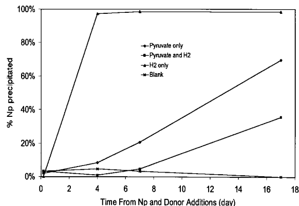
Figure 3. Fate of Np in growth experiments in which H_2 (12.3 mM) was or was not provided as an electron donor. Addition of hydrogen alone accelerated Np precipitation. Addition of hydrogen and pyruvate showed the slowest precipitation rate.
