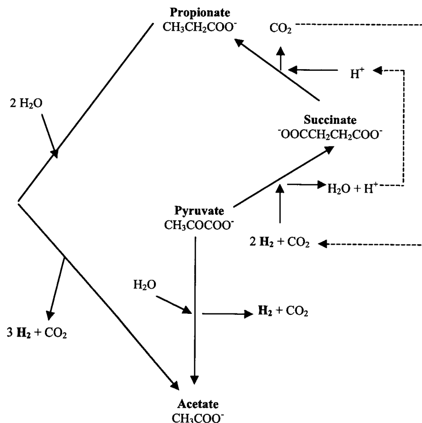
Figure 7. Alternate pathways of propionate and acetate formation from pyruvate fermentation by Desulfobulbus propionicus . A key intermediate in the propionate pathway is succinate. The \text{H}^+ and \text{CO}_2 cycling shown on the diagram (dashed arrows) represent internal transcarboxylation of propionyl-CoA to methylmalonyl-CoA. During pyruvate fermentation, high hydrogen partial pressures favor propionate formation. High hydrogen partial pressure inhibits fermentations leading to acetate. Adapted from Hansen (1993) and Madigan et al. (2000).
