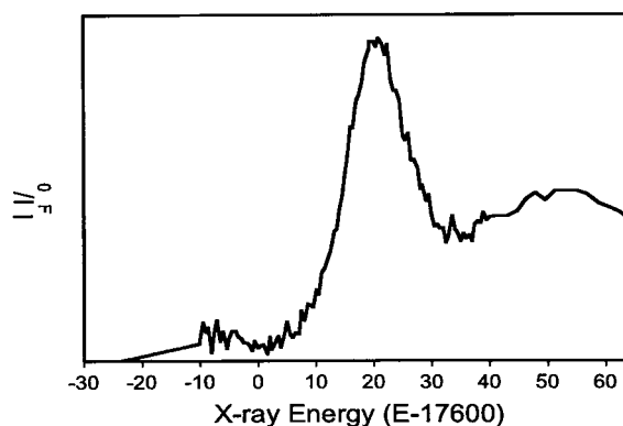
Figure 6. XANES spectra of precipitated Np from a growth experiment whose results are in Figure 2. The lack of the XANES shoulder at 25 eV associated with the linear dioxo structure of Np(V), the lack of a peak at just over 50 eV associated with Np(VI), and the peaks at 20 and 55 eV (characteristic of Np(IV)) indicate that the precipitate contained mainly Np(IV).
